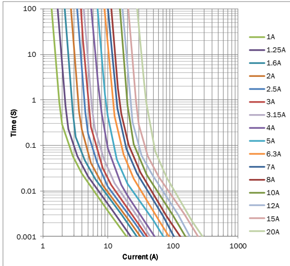
Time-Current Curve
