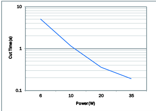
■ Various heater wattage at 25°C ambient temperature.
