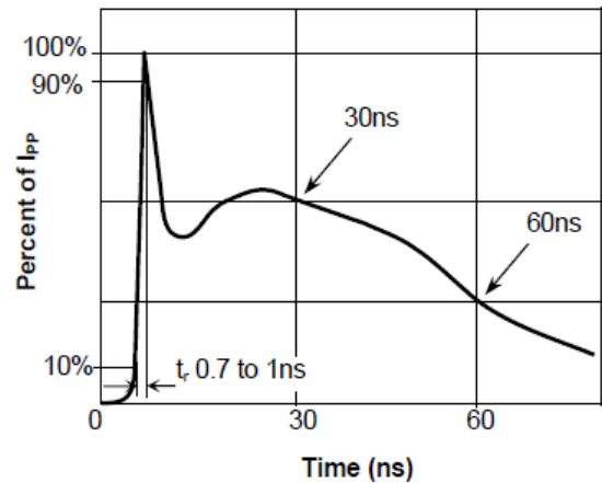
Fig.4 Pulse Waveform-ESD(IEC61000-4-2)
