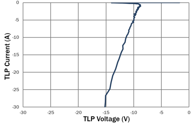
Figure 8: TLP Negative I-V Curve
