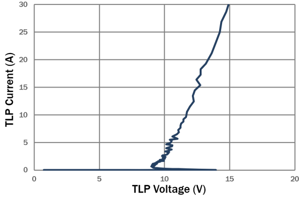
Figure 7: TLP Positive I-V Curve
